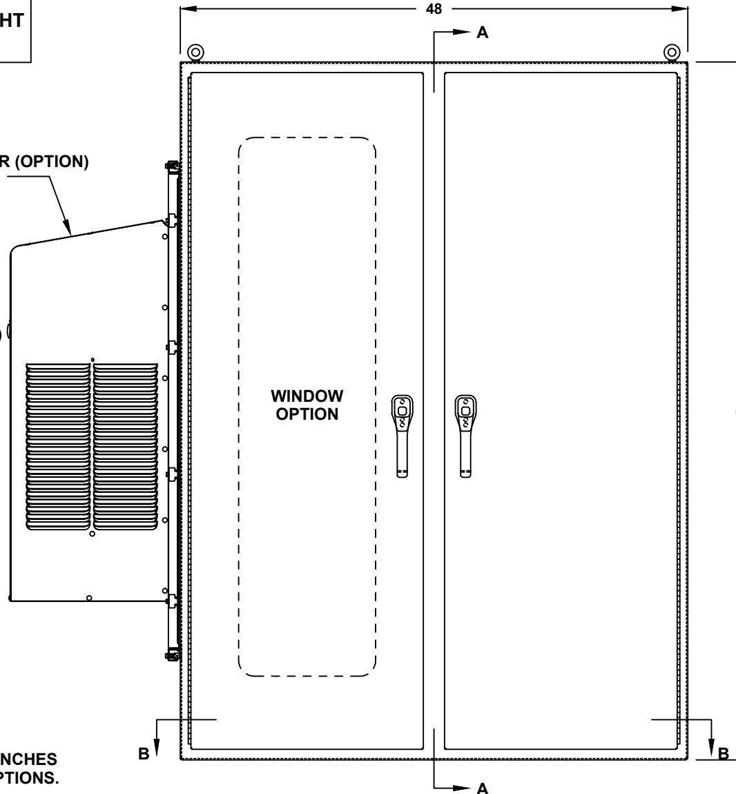
FRONT VIEW
